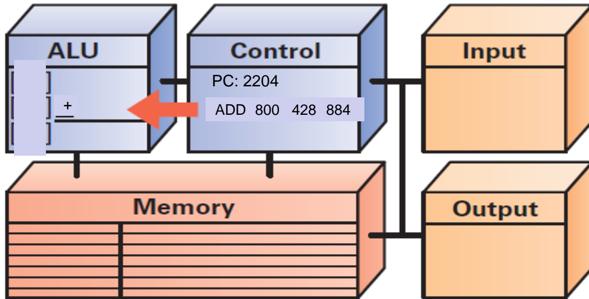
Figure 9.7 Instruction Decode: Pull apart the instruction, set up the operation in the ALU, and compute the source and destination operand addresses.
