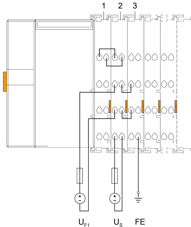
Figure 19: Power Supply Concept for Marine Applications – Classes A and B with FE Power Jumper Contact
