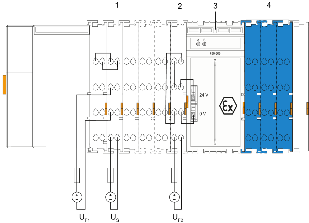
Figure 22: Power Supply Concept for Marine Applications in Ex i Zone – Class B
