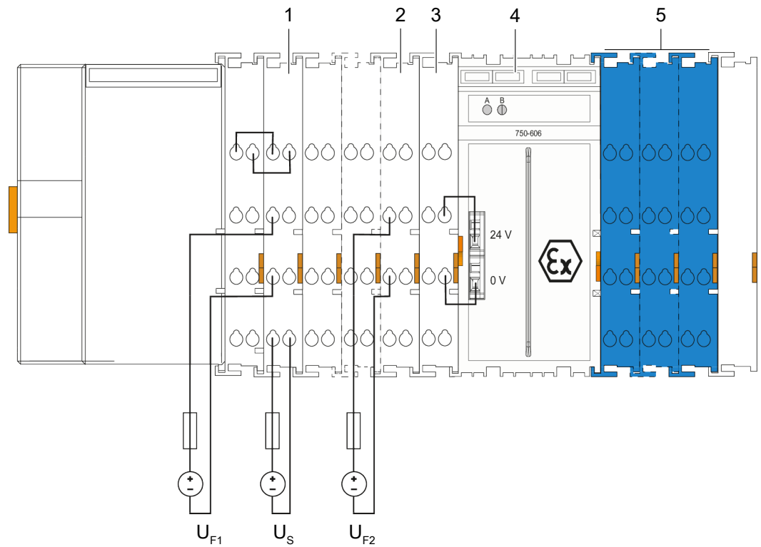
Figure 21: Power Supply Concept for Marine Applications in Ex i Zone – Class A
