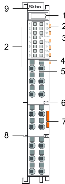
Figure 6: 750 Series I/O Module with Push-in CAGE CLAMP® Connections (Example)
