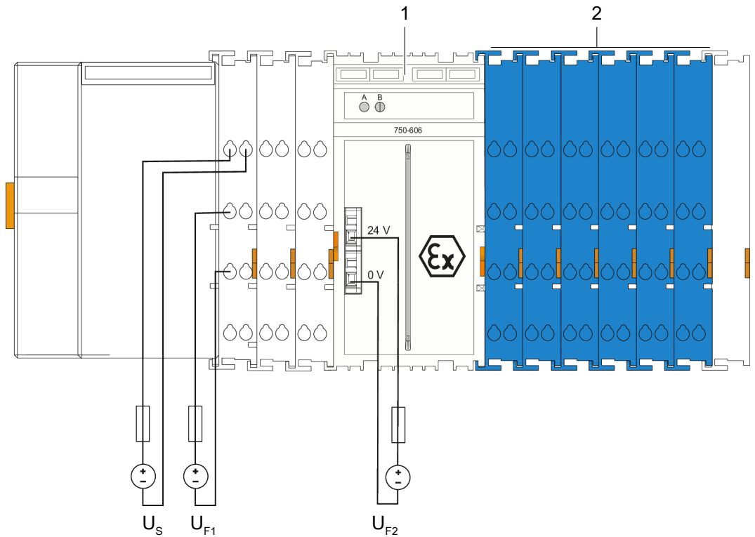
Figure 20: Ex i Power Supply Concept
