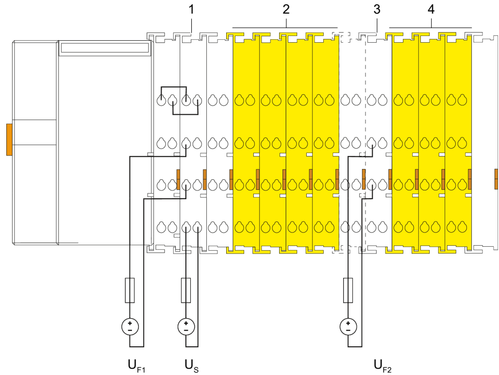
Figure 23: Power Supply Concept Example with F I/O-Modules
