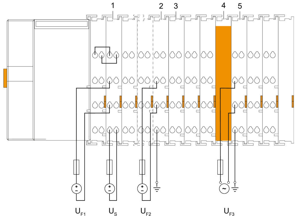
Figure 18: Power Supply Concept for Marine Applications – Classes A and B
