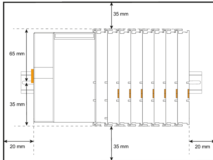
Figure 16: Installation Clearances
