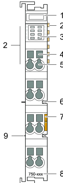
Figure 5: 750 Series I/O Module with CAGE CLAMP® Connections (Example)
