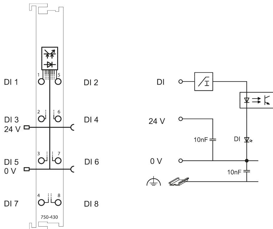
Figure 5: Circuit Diagram
