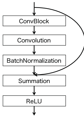
Figure 3: ResBlock architecture.
