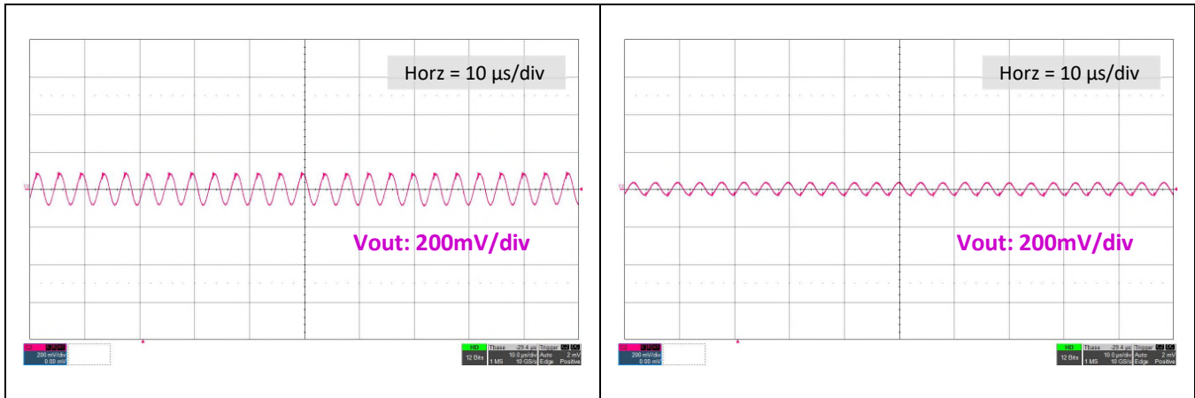
Typical Output Ripple at full load with step-up mode; Vin=10V, Vo=12V, Io=8.0A; Cext=330μF with 60mohm ESR of electrolytic capacitor.
