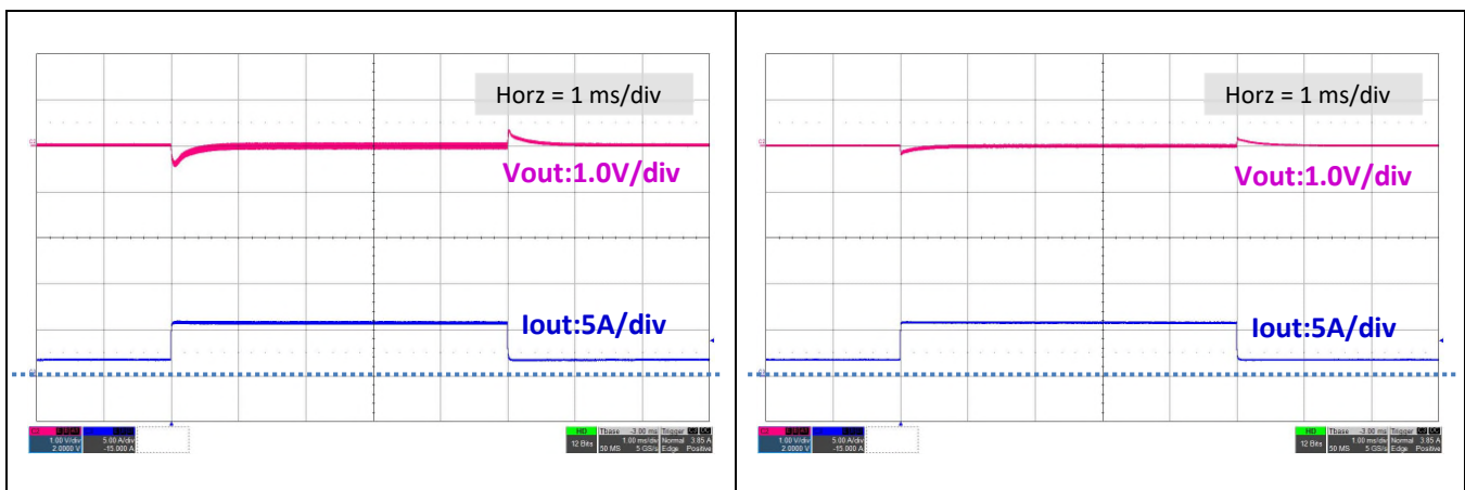
Typical Load transient response with step-up mode; Load Step from/to 25%(2A) and 75%(6A) with Slew rate of 1.0A/μs; Vin=10V, Vo=12V Cext = 330μF.
