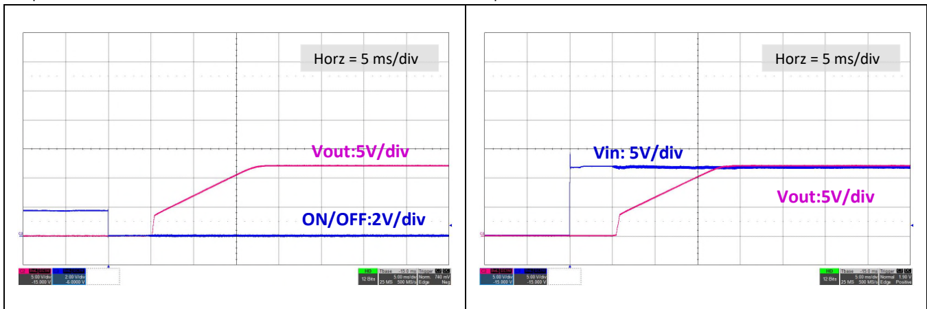
Typical startup characteristic from on/off at full load; Vin=12V, Vo=12V, Io=8.0A, Cext=330μF.
