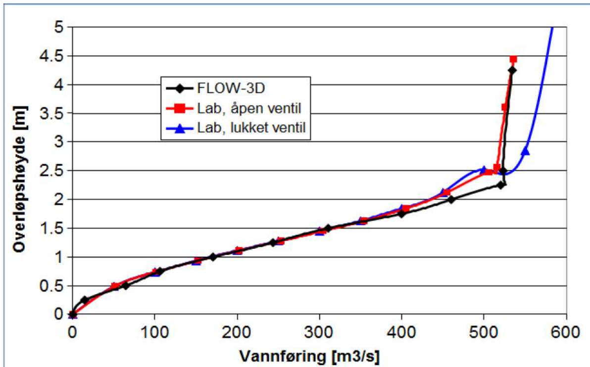
Figure 2-2: Comparison between capacity curves from simulation and physical experiment at Sysendammen (N.R.B Olsen, 2015)
