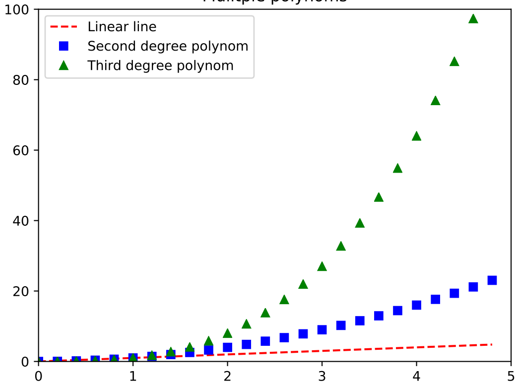
Multiple polynoms
