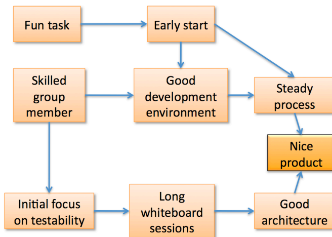
Figure 6. Positive causal map for nice product
