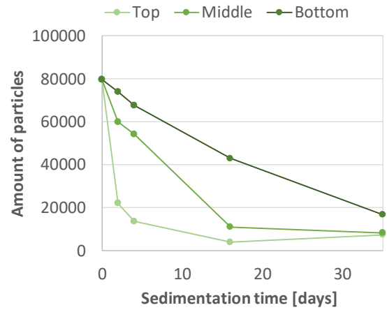
Reduction of particle concentration in the sedimentation column in dependence on sampling point and time.
