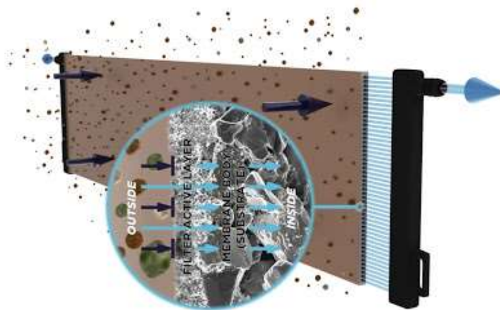
Scematic of a ceramic membrane sheet
