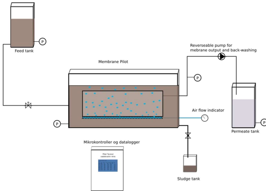
Scematic of the membrane filtration pilot
